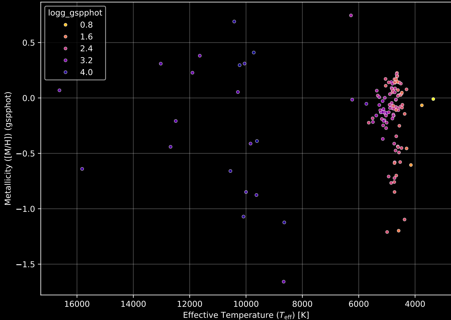
APOGEE DR17 Field: [120-08-RV] Stellar Population Parameters (n= 129)
