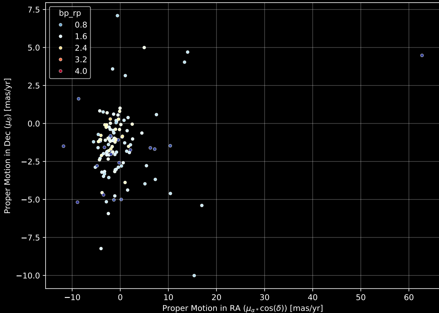
APOGEE DR17 Field: [120-08-RV] Proper Motion Diagram (n= 129)
