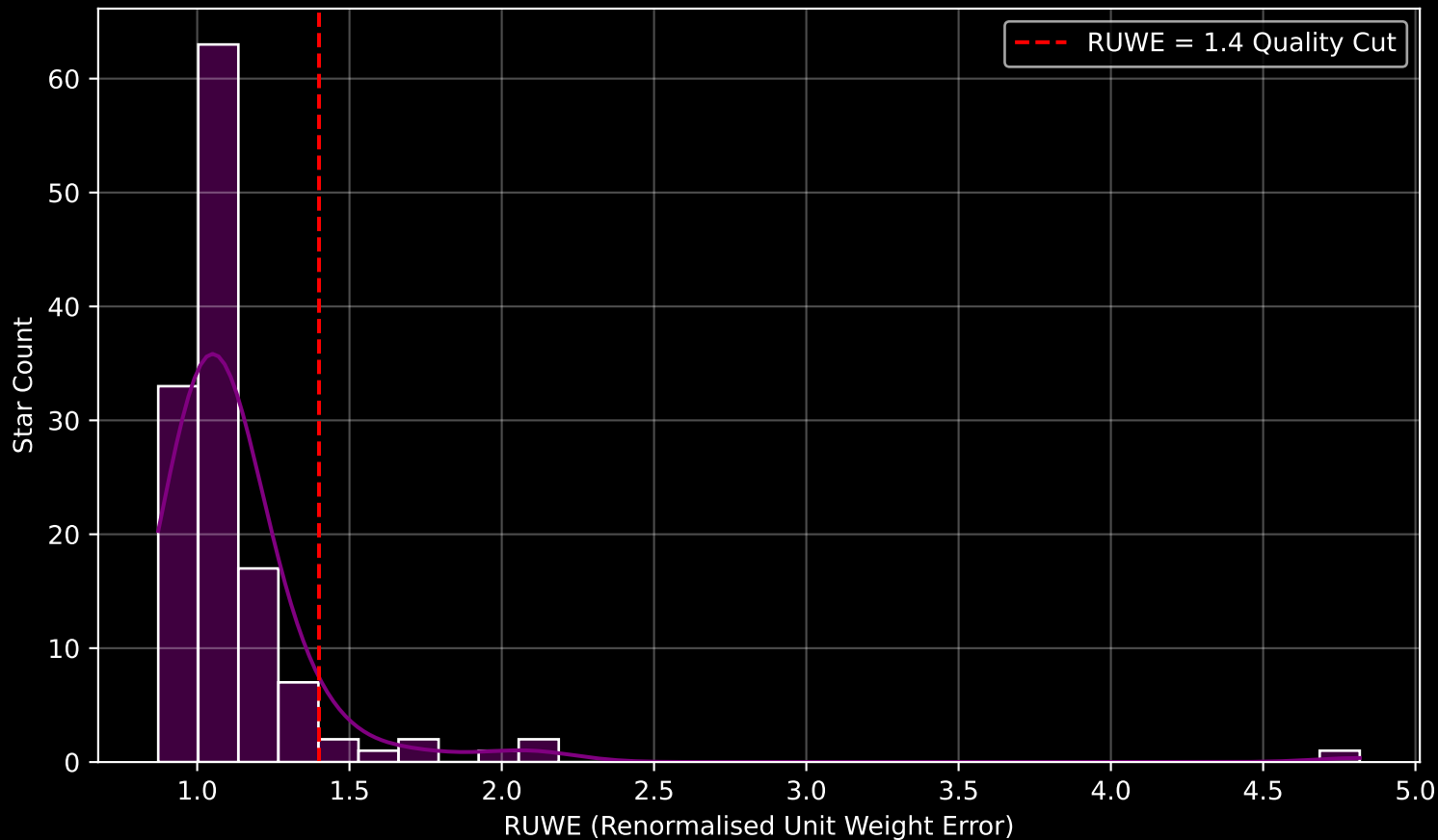
GAPOGEE DR17 Field [120-08-RV] RUWE Distribution (n= 129)
