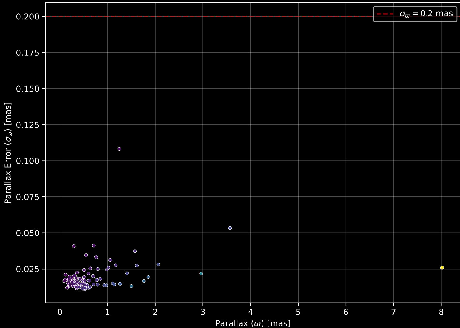
APOGEE DR17 Field: [120-08-RV] Parallax Quality (n= 129)
