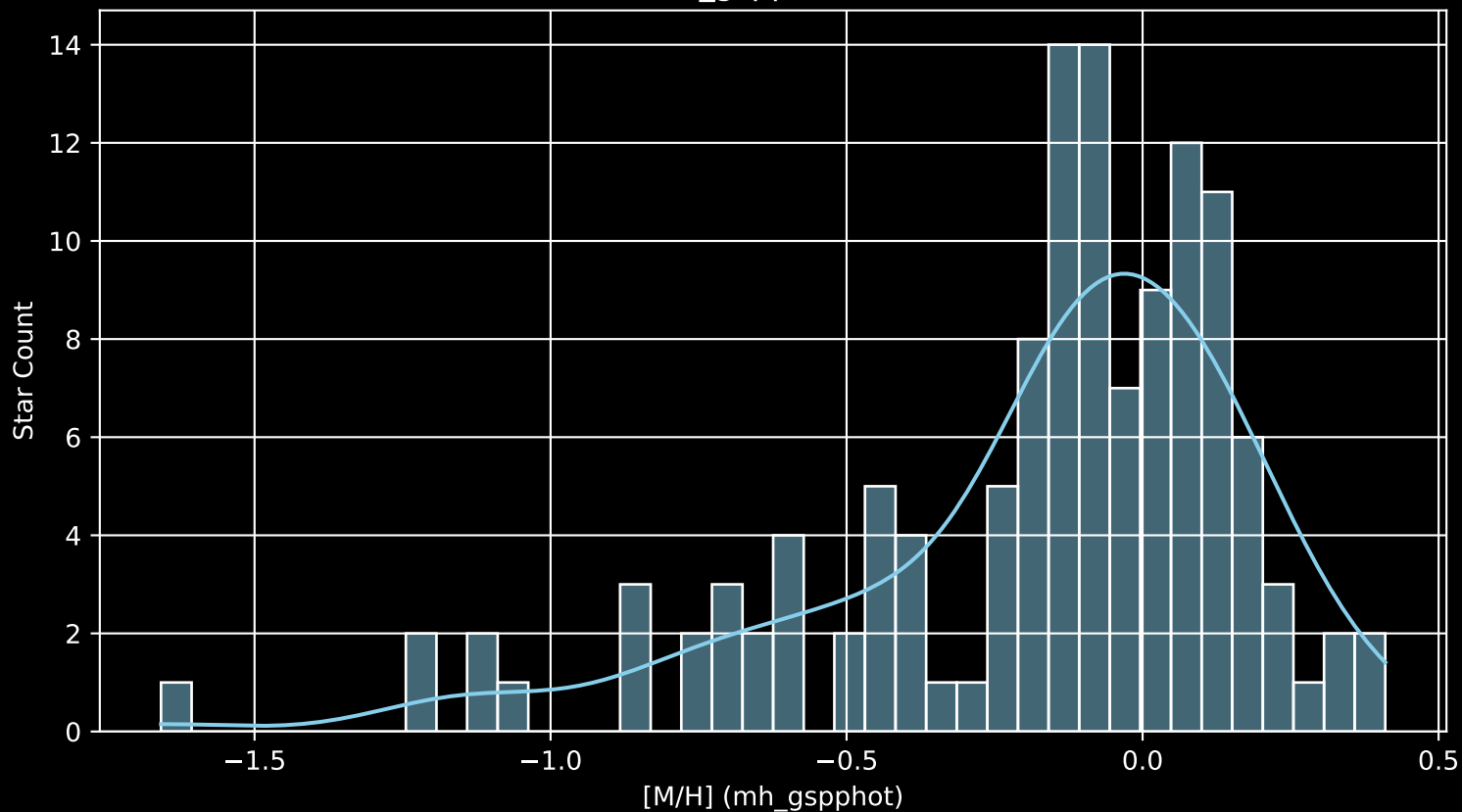
APOGEE DR17 Field: [120-08-RV [M/H] (mh_gspphot) (n= 127)
