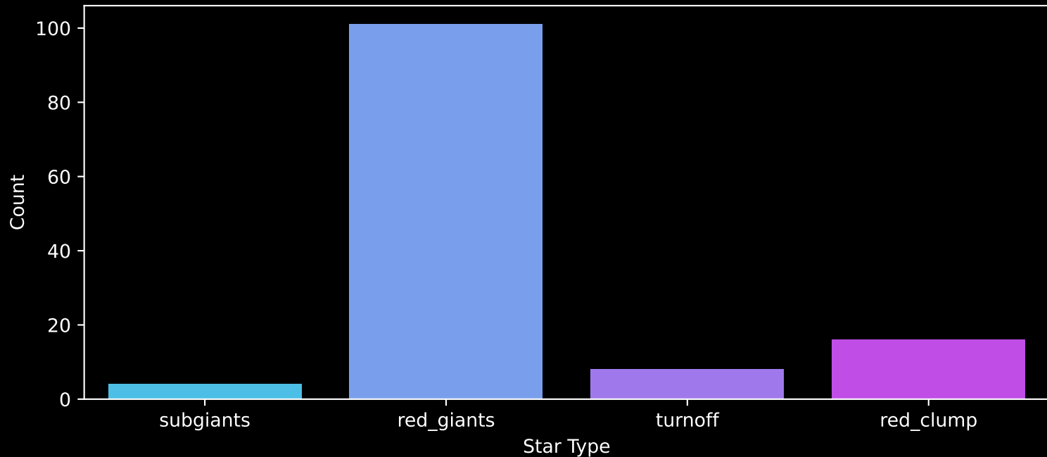
APOGEE DR17 Field: [120-08-RV] Count plot of Star Type
