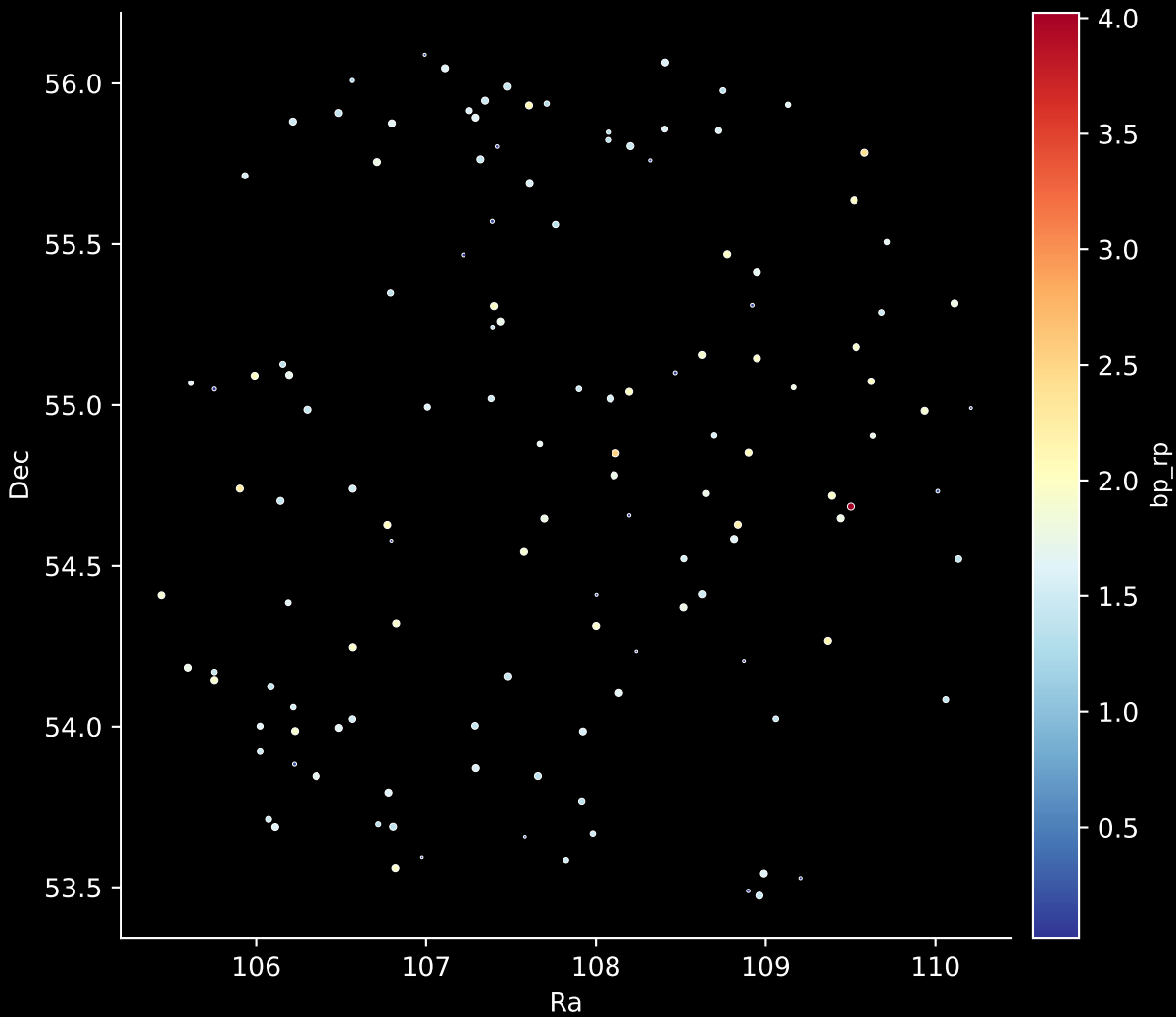
APOGEE DR17 Field: [120-08-RV] Stars: 129
